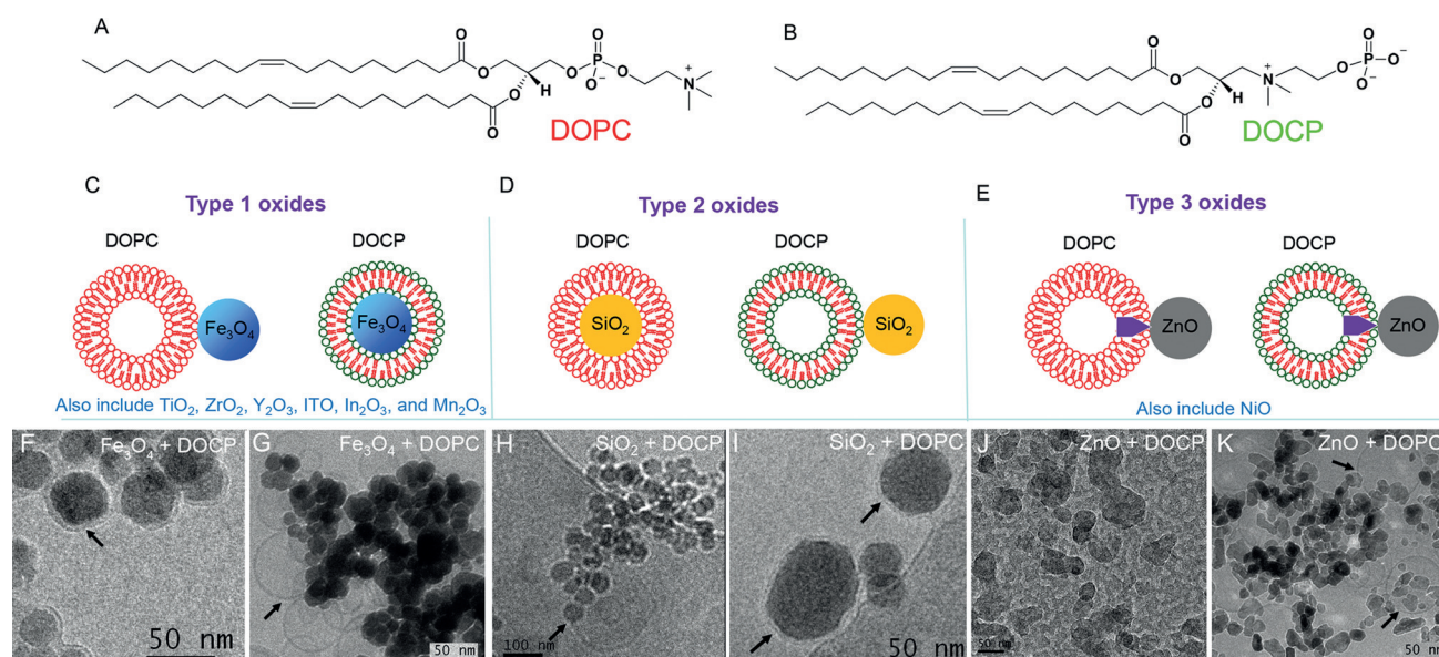
Figure 1. The structures of A) DOPC and B) DOCP lipids. The three types of metal oxides based on their lipid interactions: C) Type 1 includes \text{Fe}_3\text{O}_4 , \text{TiO}_2 , \text{ZrO}_2 , \text{Y}_2\text{O}_3 , ITO, \text{In}_2\text{O}_3 , and \text{Mn}_2\text{O}_3 ; they are adsorbed by DOPC, but form supported bilayers with DOCP. D) Type 2 includes only \text{SiO}_2 , forming supported bilayers with DOPC. E) Type 3 includes cationic \text{ZnO} and \text{NiO} , damaging the membranes (pores indicated by the blue color); full membrane disruption occurs to DOCP when mixed with \text{ZnO} . Cryo-TEM images of F), G) \text{Fe}_3\text{O}_4 , H), I) \text{SiO}_2 , and J), K) \text{ZnO} NPs mixed with F), H), J) DOCP or G), I), K) DOCP liposomes. In each sample, the liposomes were added in excess and the free liposomes were removed after centrifugation and washing before cryo-TEM; see the Supporting Information for details. The arrowheads point at the lipid features.
