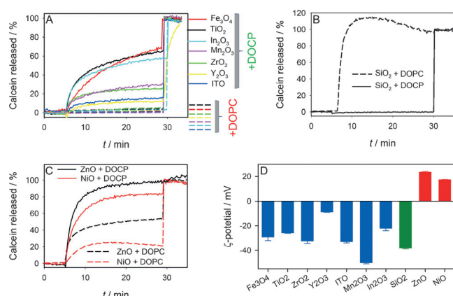
Figure 2. Calcein leakage from the DOPC and DOCP liposomes induced by adding A) \text{Fe}_3\text{O}_4 , \text{TiO}_2 , \text{ZrO}_2 , \text{Y}_2\text{O}_3 , ITO, \text{In}_2\text{O}_3 , or \text{Mn}_2\text{O}_3 ; B) \text{SiO}_2 ; and C) \text{ZnO} and \text{NiO} NPs. Solid lines: mixed with DOCP; dashed lines: mixed with DOPC. Oxides were added at 5 min and Triton X-100 at 30 min in buffer (10 mM HEPES, pH 7.4 with 100 mM NaCl), except for \text{In}_2\text{O}_3 , ITO, \text{Mn}_2\text{O}_3 with 300 mM NaCl. D) \zeta -potential of the oxides in 10 mM HEPES, pH 7.4 at 25°C.
